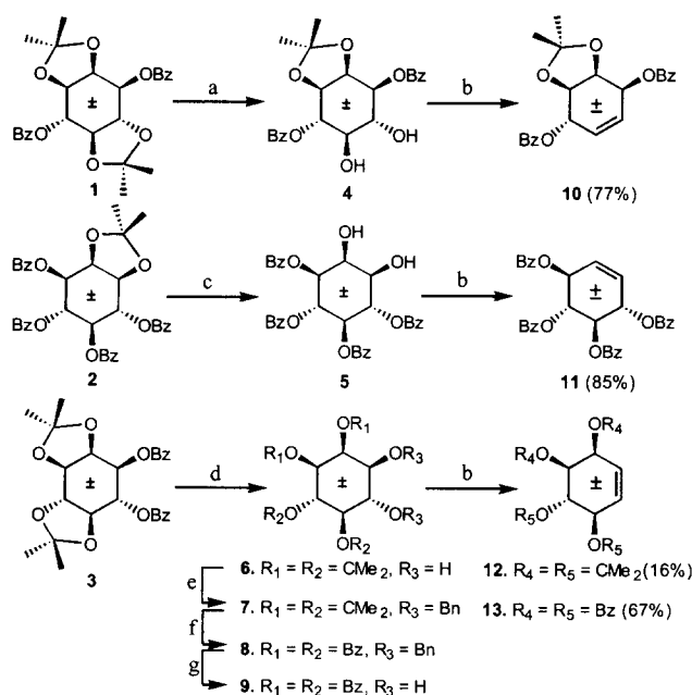
Scheme 1. Reagents and conditions: a. \text{AcCl} (cat.), \text{CH}_2\text{Cl}_2/\text{MeOH} , 75%; b. see Table 1; c. 80% aq. \text{AcOH} , 100 °C, quant.; d. \text{NaOMe} , \text{MeOH} , \uparrow\downarrow , 95%; e. \text{BnBr} , \text{NaH} , \text{DMF} , 92.6%; f. i) 80% aq. \text{AcOH} , 100 °C, ii) \text{BzCl} , pyridine, 94%; g. \text{Pd}(\text{OH})_2/\text{C} , \text{H}_2 (50 psi), \text{EtOAc}/\text{EtOH} , 97%.
