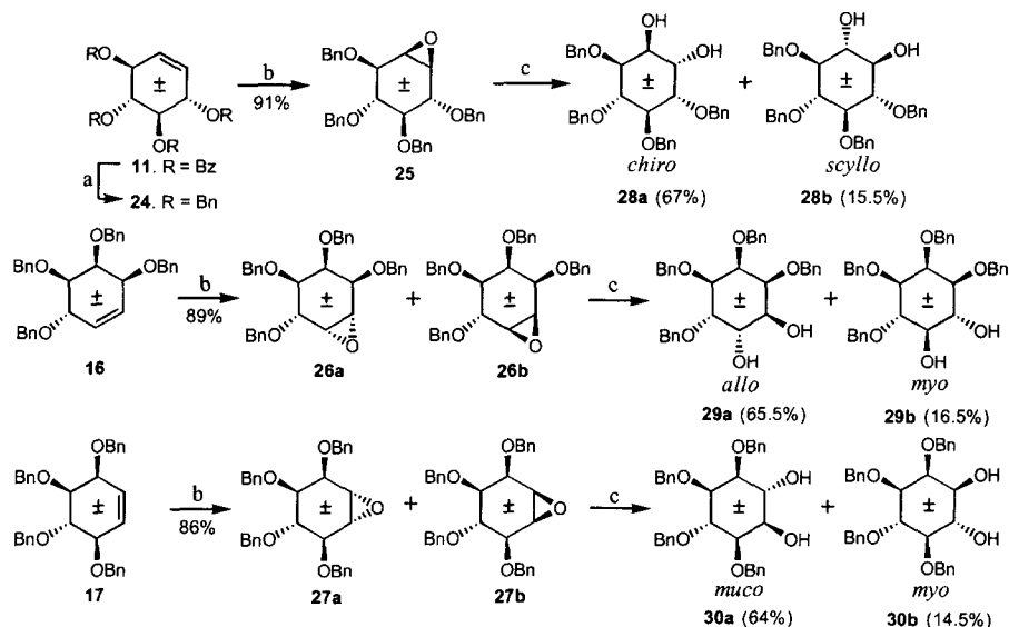
Scheme 3. Reagents and conditions: a. i) NaOMe, MeOH, \uparrow\downarrow , ii) BnBr, NaH, DMF, 91%; b. I 2 , Ag 2 O, aq. dioxane, 90 °C; c. CF 3 COOH (or H 2 SO 4 ), aq. THF, 50 °C.
